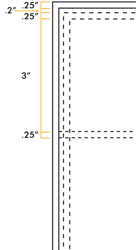
TOP AND BOTTOM POLE POCKET DETAIL MEASUREMENTS
